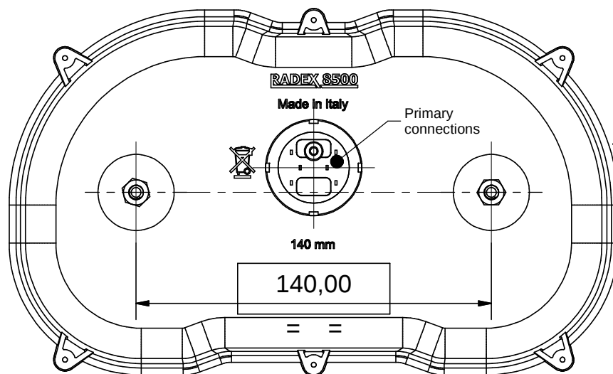
- REAR VIEW LAMP - Scale (1:2)
